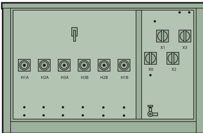
» 3. Live Front Loop Feed
