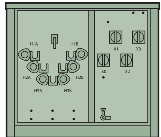
» 4. Dead Front Loop Feed
