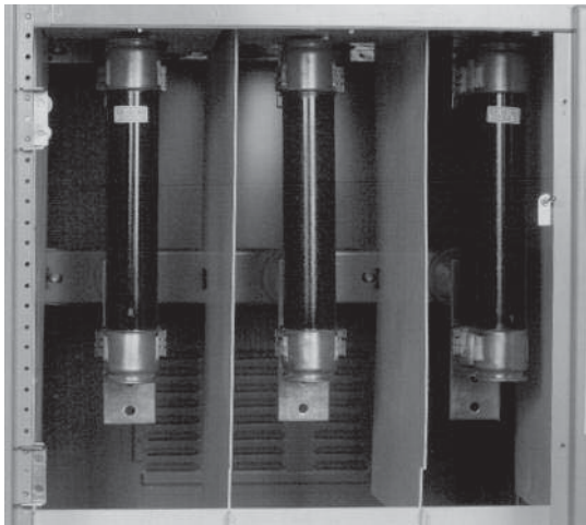
Figure 16 Installed Fuses
