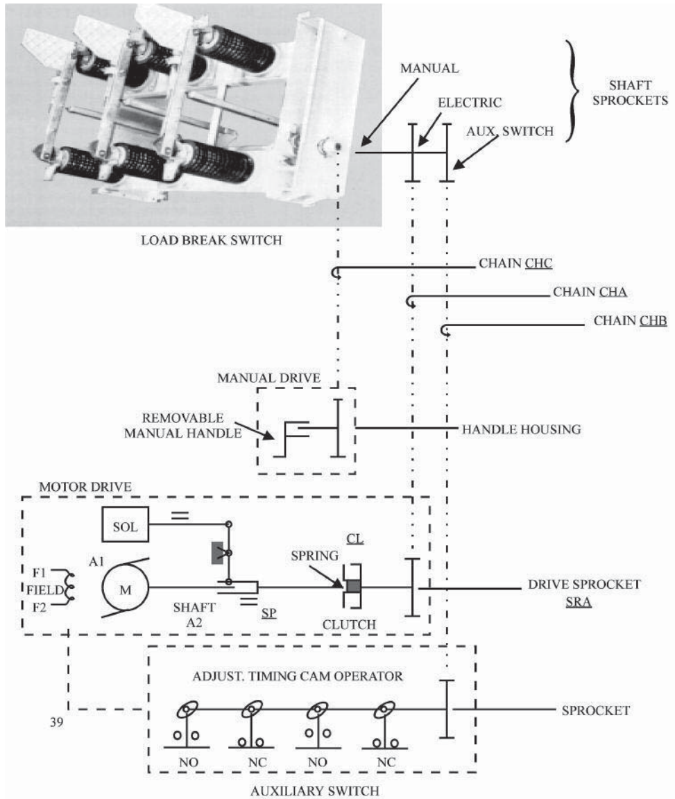
Figure 18 Motor Drive System Kinematic Diagram
